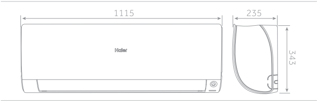
MOUNTING DIMENSIONS
