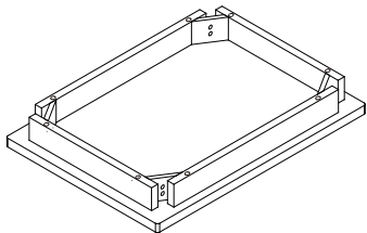
④ x1 495X360X65mm
