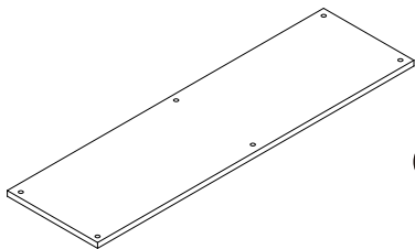
⑧ x1 955X288X12mm
